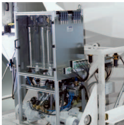
Admixture weighing system for chemical additives.
