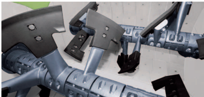
The robust and high-capacity mixing unit is designed to be particularly energy saving.
